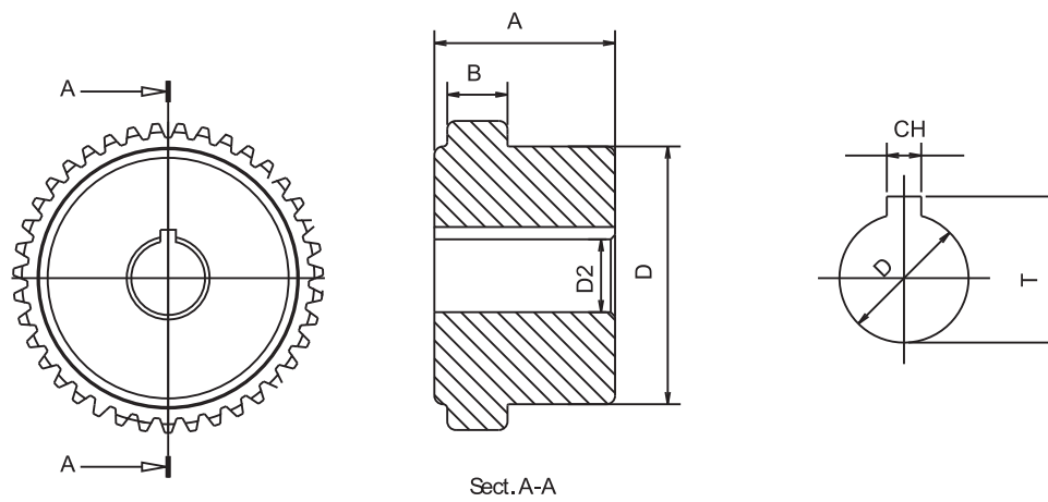
Sect. A-A
