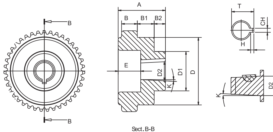
Sect. B-B
